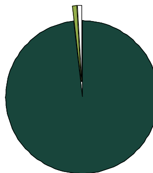
Figure 1 Unresolved 1% Unplaced 1%
